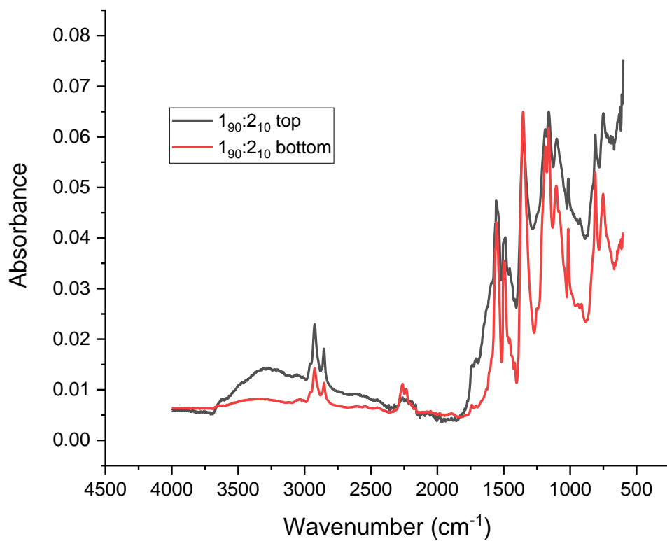
Figure S1: IR spectra of top and bottom of [1 90 :2 10 ] blend.
