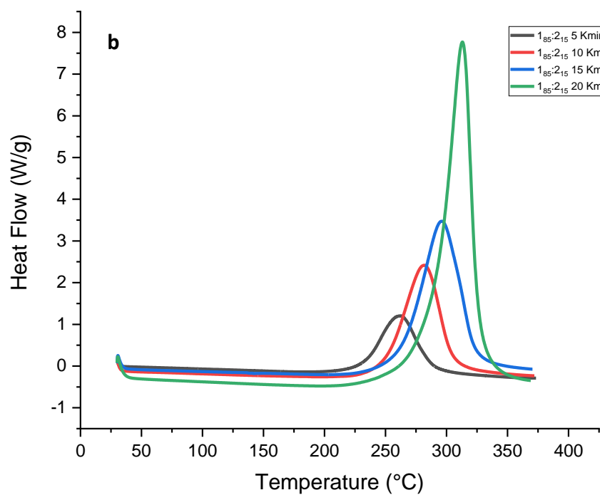
Figure S2: DSC thermograms of selected compounds: 1 (a) and 1 85 :2 15 (b) at different heating rates.
