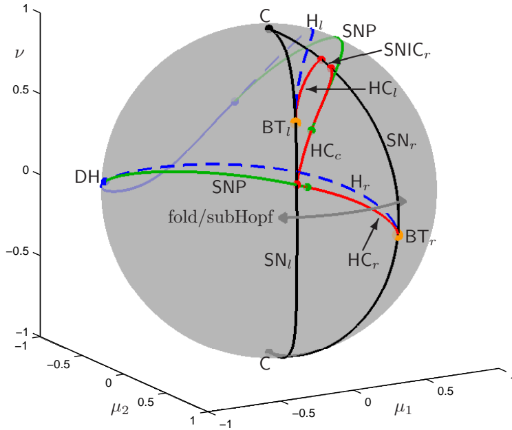
Figure 2: Bifurcation diagram of system (3) with b = 0.75 on the unit sphere in (\mu_1, \mu_2, \nu) -space. Color in on-line version: red, homoclinic (HC); blue, Hopf bifurcation (H; solid: supercritical, dashed: subcritical); black, saddle-node (SN); orange, Bogdanov–Takens point (BT); green, saddle node of periodics (SNP); degenerate Hopf and cusp are labeled DH and C, respectively. A path of pseudo-plateau bursting is indicated; we used the circle segment on the unit sphere with \nu = 0.1 and \mu_1 = \sqrt{1 - \nu^2} \cos(2\pi\vartheta) , where \vartheta varies between 0.245 \pm 0.065 .
