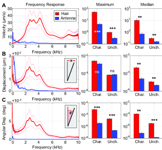
Fig. 2. Antenna (blue) and hair (red) motion in response to 10Hz-10kHz electrical chirps. Rows show the velocity (top), displacement (middle) and angular displacement (bottom). Columns show the response at each frequency (left), the amplitude of maximum response (middle) and the median response amplitude across all frequencies (right). Insets show a representation of the quantity being measured.
