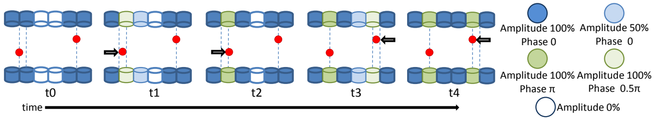
Figure 4: Individual movement of two beads in opposing directions. At time t_0 both beads are stationary. At time t_1 , the phase of the second column of transducers increases from 0 to 0.5\pi and the amplitude of the third column of transducers increases from 0 to 50%; resulting in a movement of the left bead towards the centre. At time t_2 , a similar increase in phase and amplitude leads to continued movement for the left bead. At time t_3 and t_4 , the same change occurs on the right side to move the second bead towards the centre. The step size in amplitude and phase determines the amount of movement.
