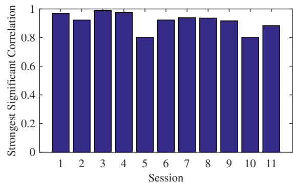
Fig. 4. Strongest significant correlation ( p < 0.05 ) in each of the sessions. The results demonstrate that physical activity information leaks consistently in different sessions that capture various activities of daily living. Each session number corresponds to the session number shown in Table I.
